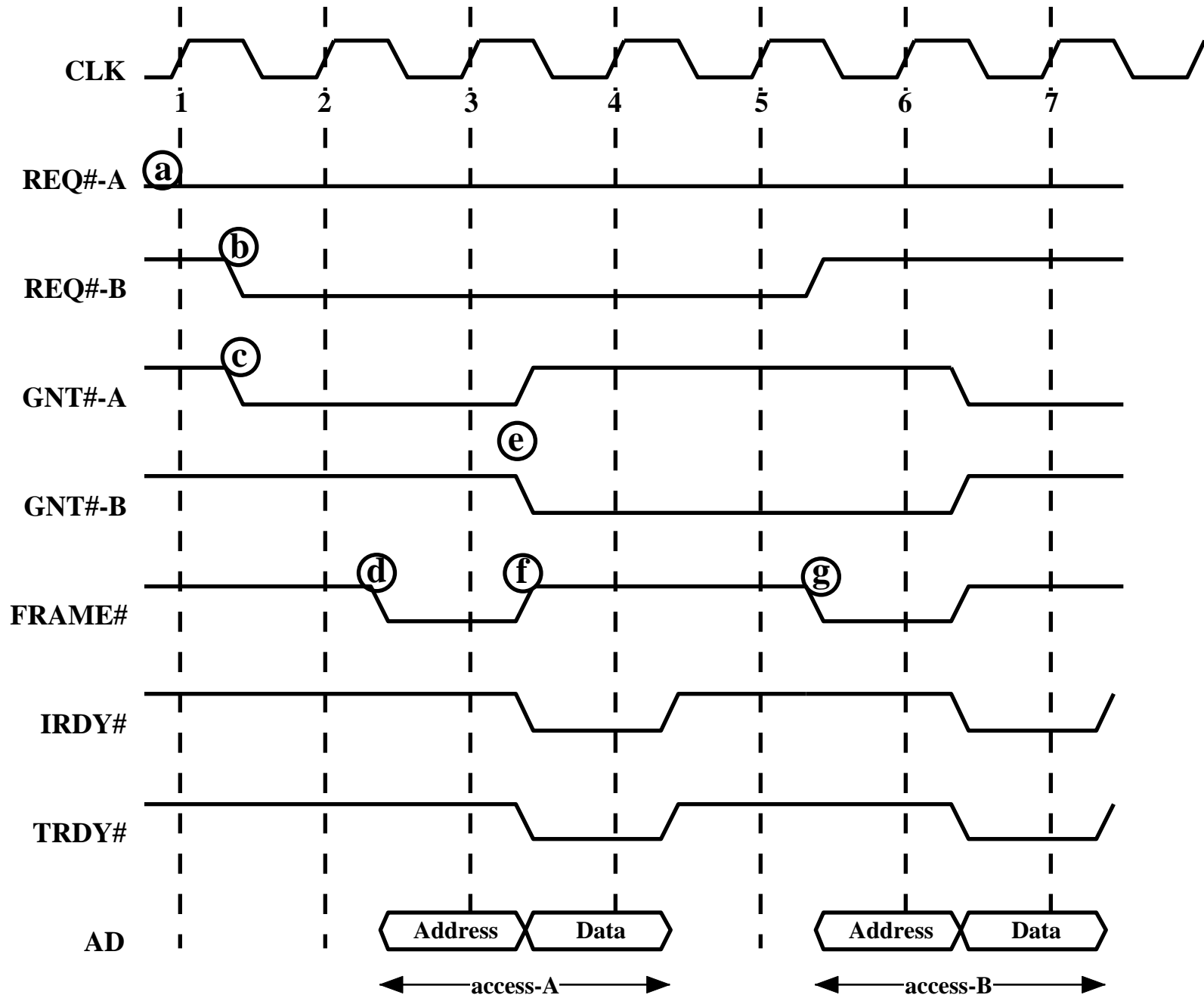
Figure 3.24 PCI Bus Arbitration Between Two Masters
